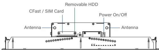
Front I/O
