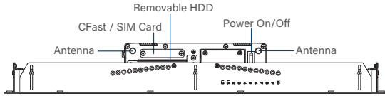
Front I/O
