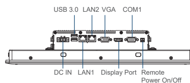
Rear I/O
