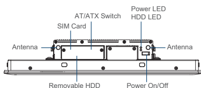
Front I/O
