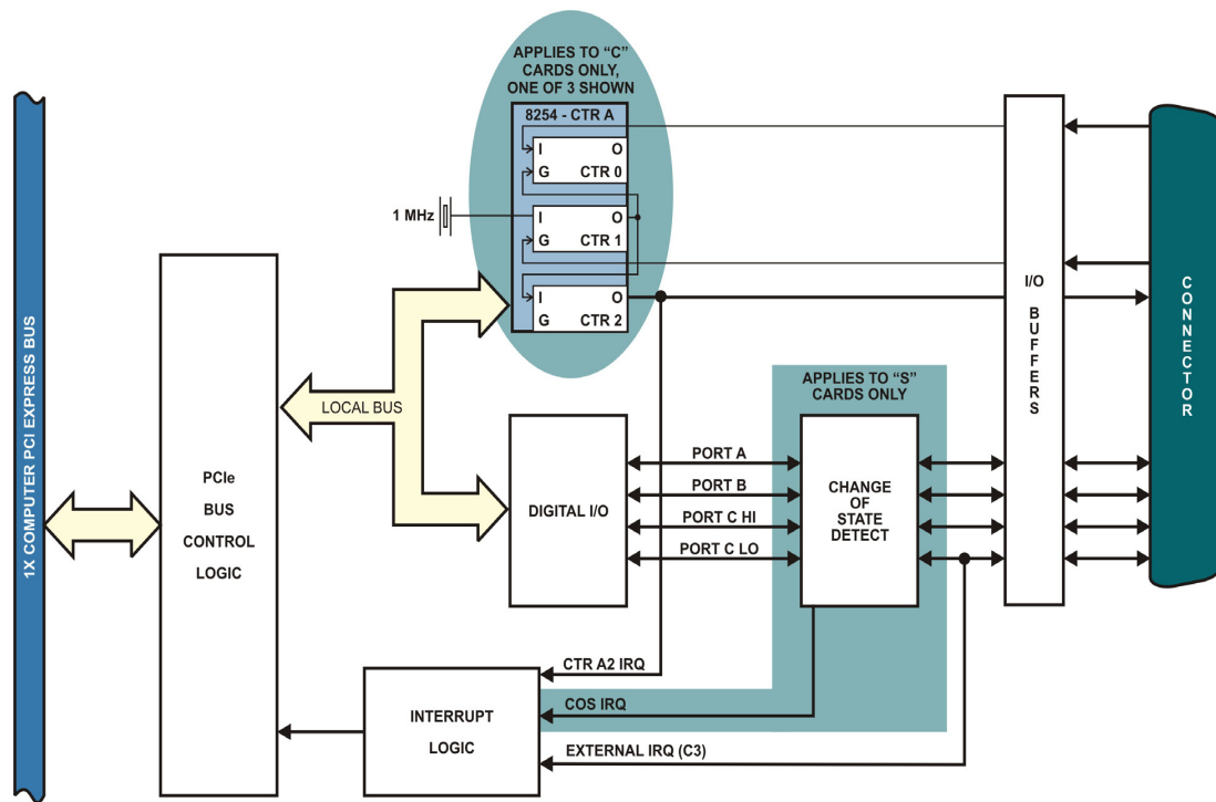
BLOCK DIAGRAM
