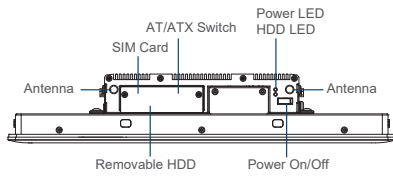
Front I/O
