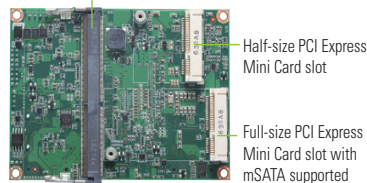
▲ Rear view
