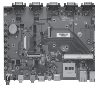
▲ Q7B120
