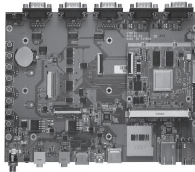
▲ Q7M120-120-EVK
