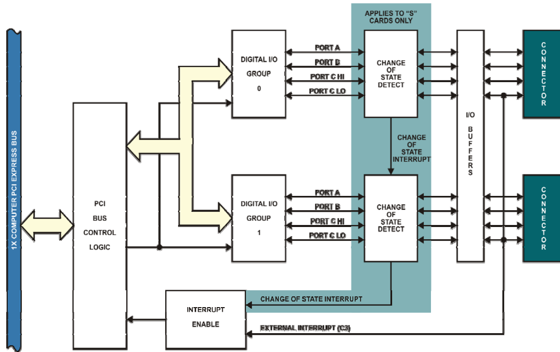
BLOCK DIAGRAM
