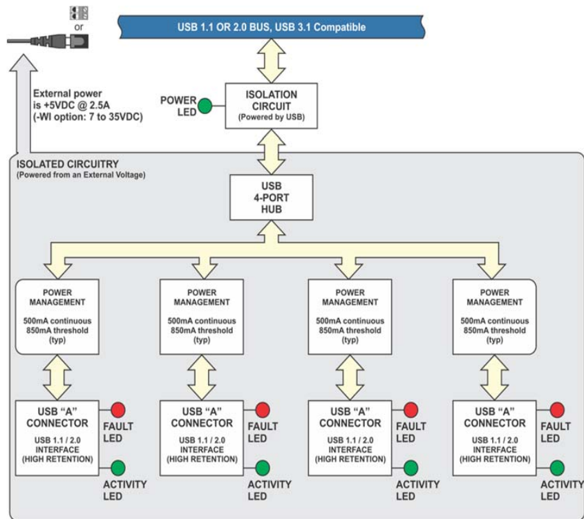
BLOCK DIAGRAM
